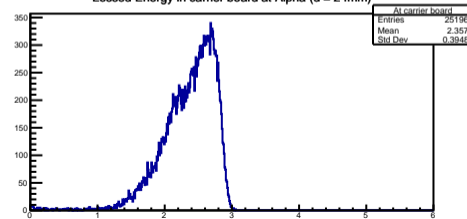
Lossed Energy in carrier board at Alpha (d = 24mm)
