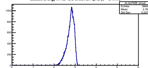
Lossed Energy in ALPIDE circuit at Alpha (d = 24mm)
